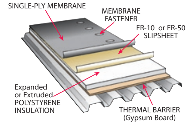
Typical Steel Deck and Polystyrene Insulation
