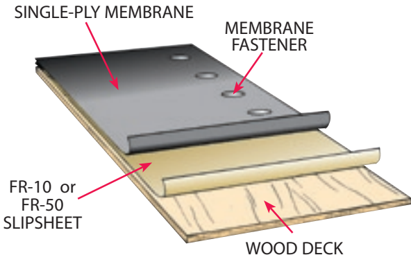
Typical Combustible Deck Application
