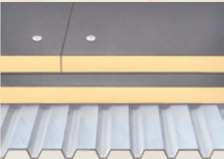
Multi-layer Application: A two layer application of ACFoam® is strongly recommended. Atlas recommends a maximum 2.7" thick top layer. Refer to Technical Bulletin #01-00 on www.atlasroofing.com .
