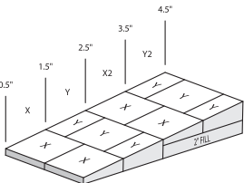
Typical cross-section of 1/4" slope with 1/2" start. Shown above as 4 panels @ 4'-0" each = 16'-0" run.
