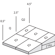
Typical cross-section of 1/2" slope with 1/2" start. Shown above as 2 panels @ 4'-0" each = 8'-0" run.
